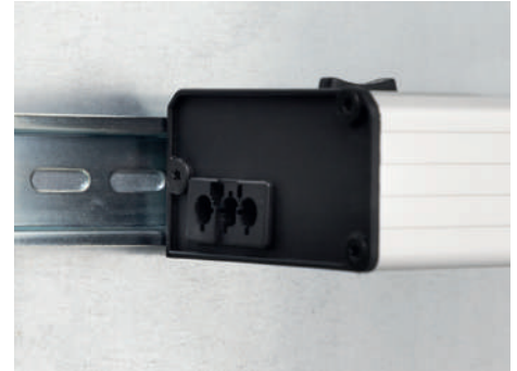
Assembly on 35 mm top hat DIN rails
