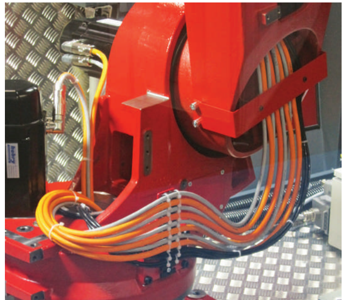
ZL 180 Robotics
