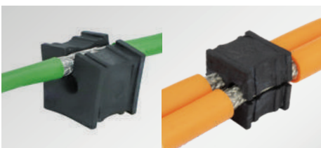
Split EMC grommets small, single and multi for cables with and without connectors for cable diameters 2 to 16 mm
